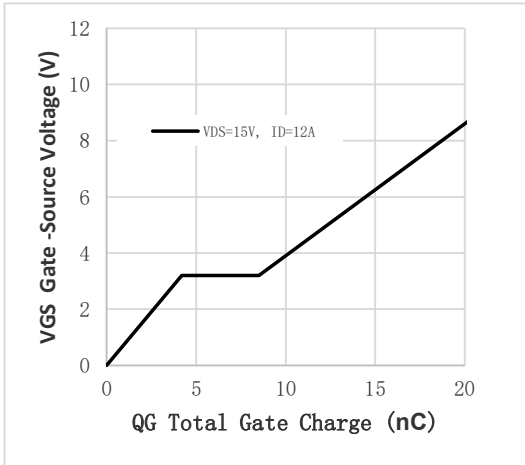
Fig.1 Gate-Charge Characteristics
