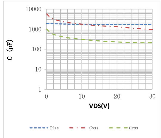
Fig.2 Capacitance Characteristics
