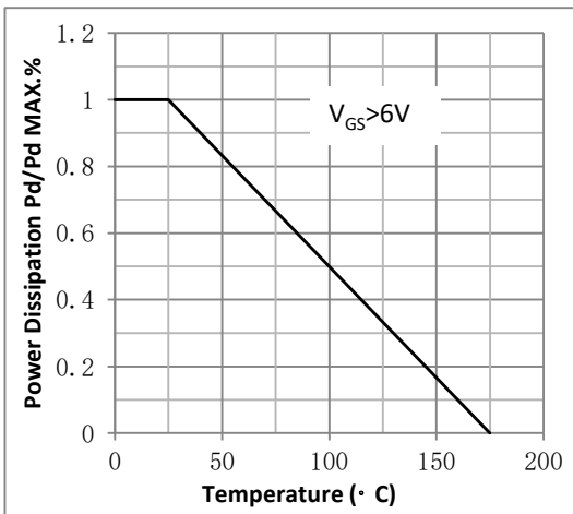
Fig.3 Power Dissipation
